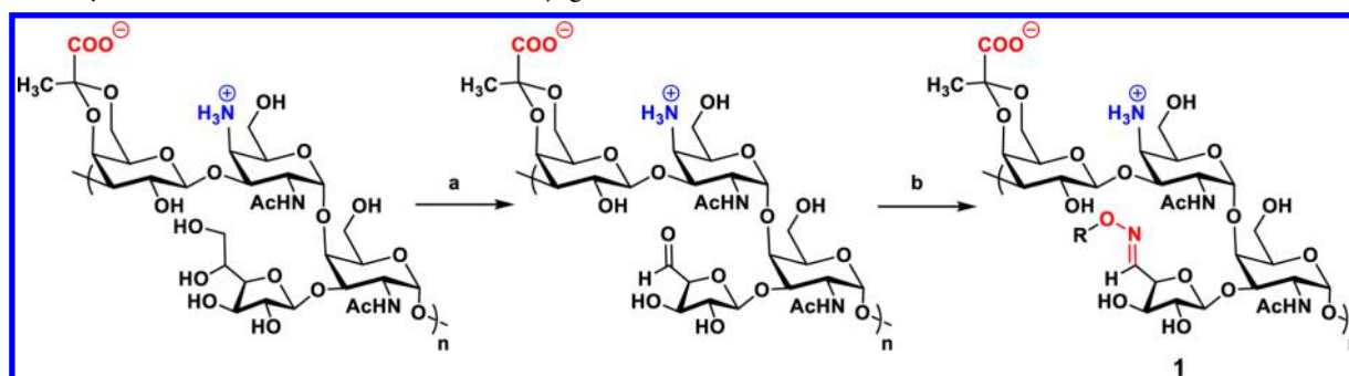
Scheme 4. Synthesis of Tetrasaccharide-PS A1 Conjugate 1 a
